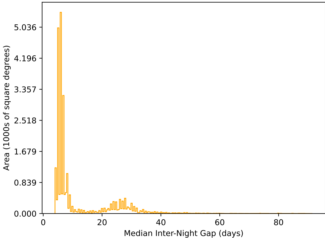
too_elab_r64_d2_gz_v3.4_10yrs All sky r band: Median Inter-Night Gap
