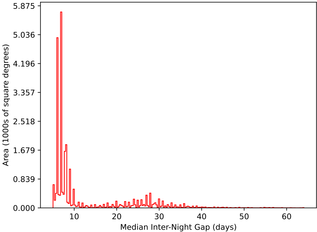
too_elab_r64_d2_gz_v3.4_10yrs All sky i band: Median Inter-Night Gap
