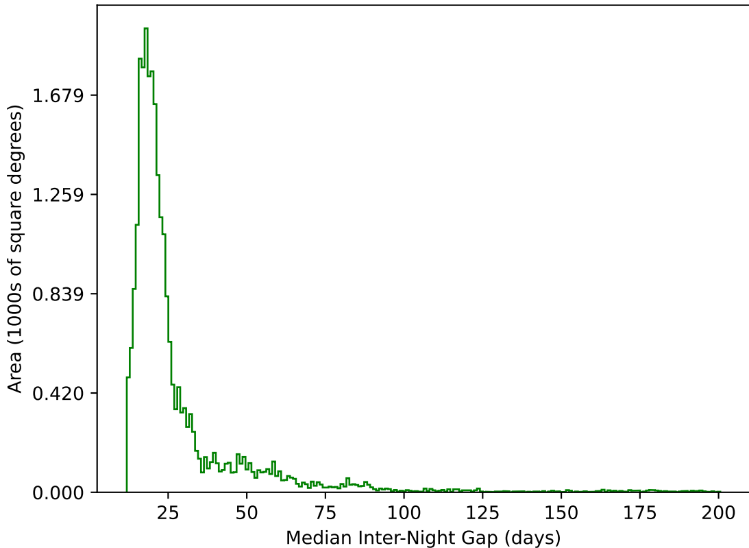
too_elab_r64_d2_gz_v3.4_10yrs All sky g band: Median Inter-Night Gap
