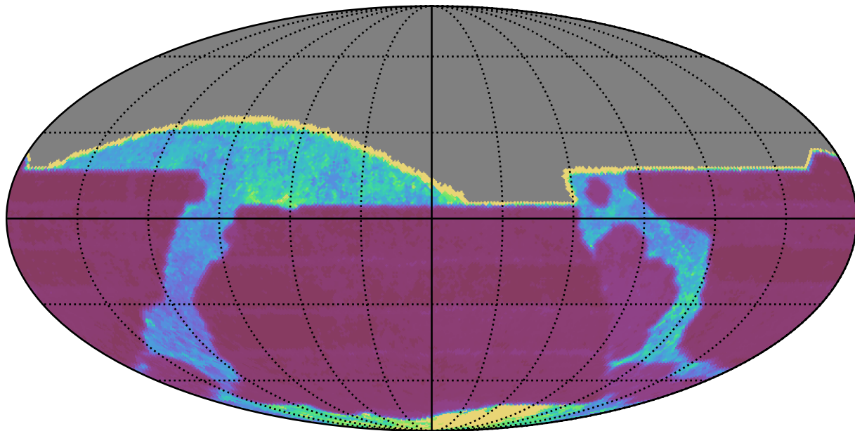
too_elab_r64_d2_gz_v3.4_10yrs All sky all bands: Median Inter-Night Gap
