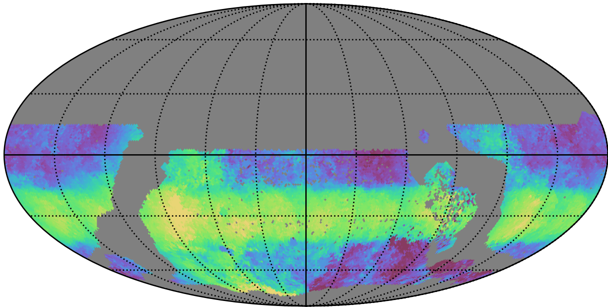
too_elab_r64_d2_gz_v3.4_10yrs WFD u band: Median HA
