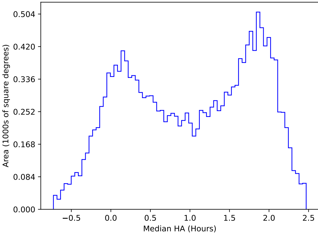
too_elab_r64_d2_gz_v3.4_10yrs WFD u band: Median HA
