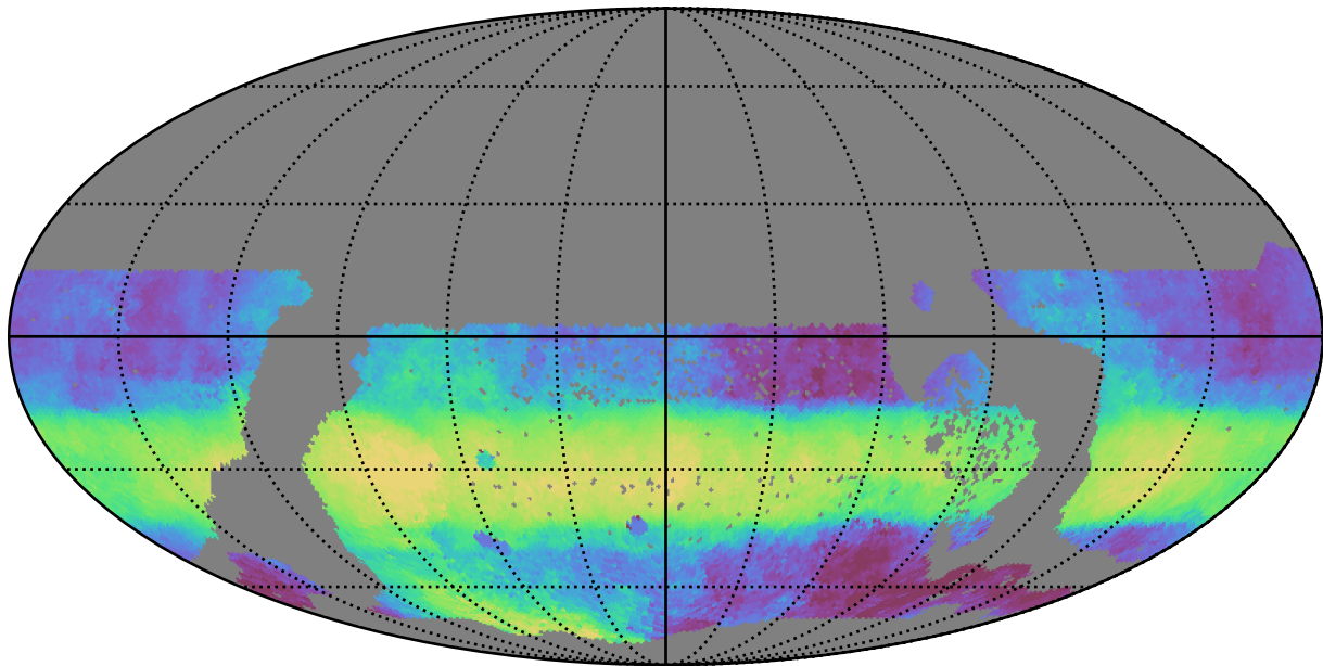
too_elab_r64_d2_gz_v3.4_10yrs WFD r band: Median HA
