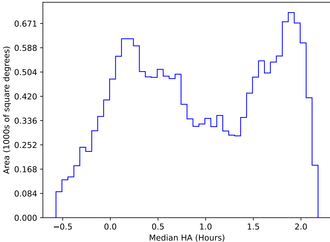
too_elab_r64_d2_gz_v3.4_10yrs WFD r band: Median HA
