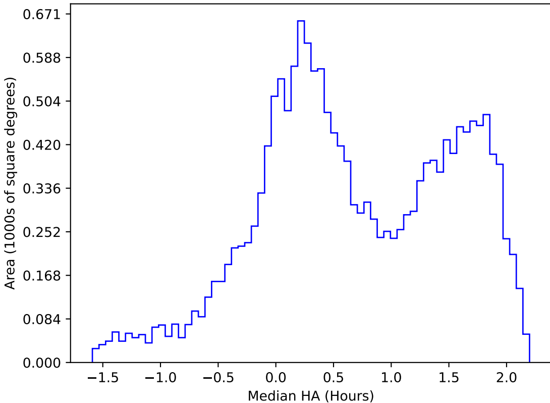
too_elab_r64_d2_gz_v3.4_10yrs WFD g band: Median HA
