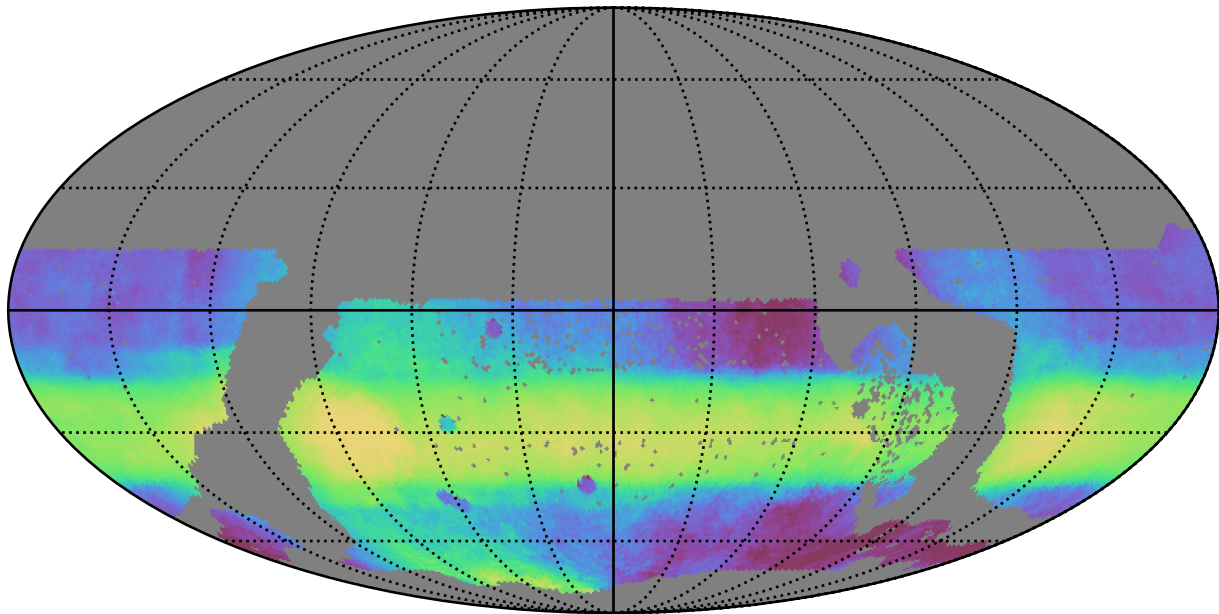
too_elab_r64_d2_gz_v3.4_10yrs WFD all bands: Median HA
