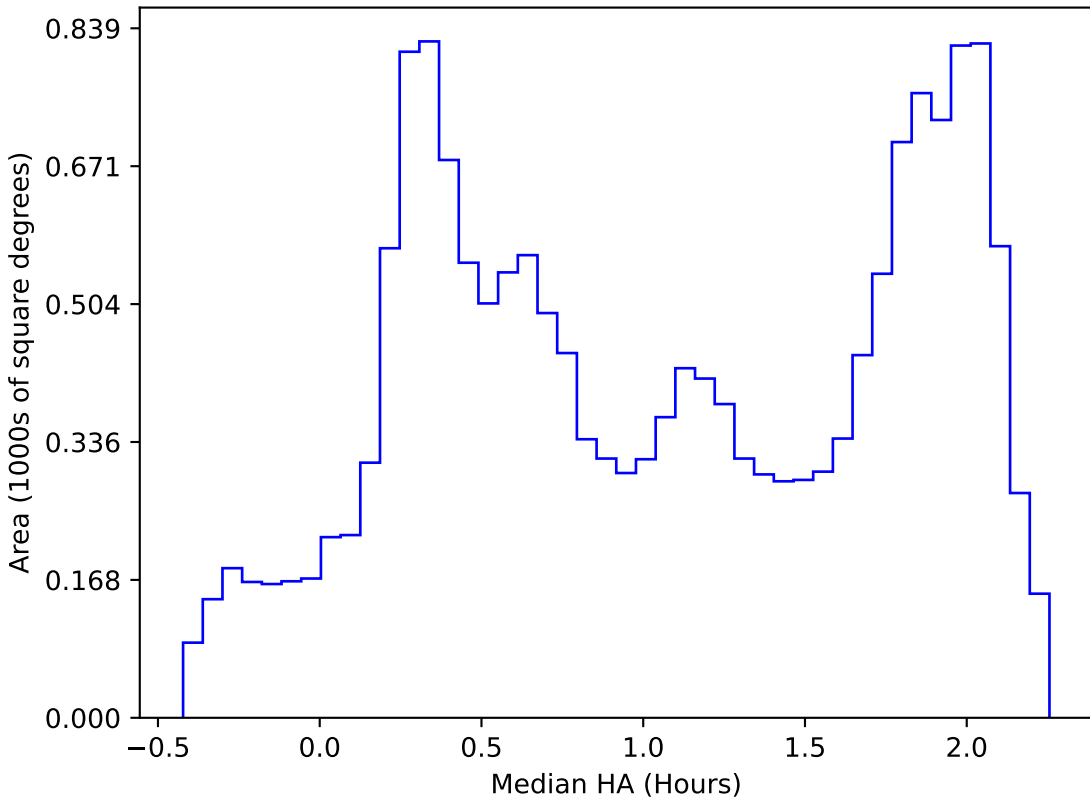
too_elab_r64_d2_gz_v3.4_10yrs WFD all bands: Median HA
