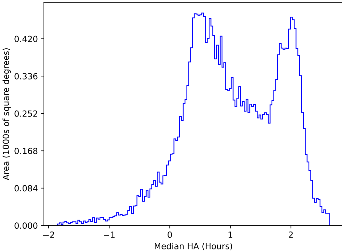
too_elab_r64_d2_gz_v3.4_10yrs All sky z band: Median HA
