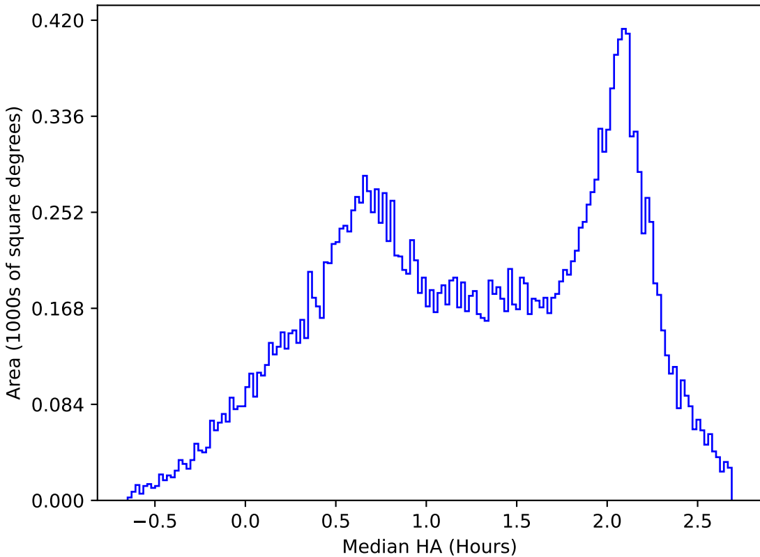
too_elab_r64_d2_gz_v3.4_10yrs All sky y band: Median HA
