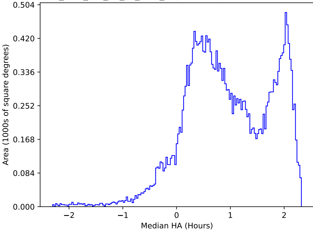
too_elab_r64_d2_gz_v3.4_10yrs All sky i band: Median HA
