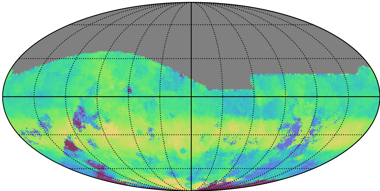
too_elab_r64_d2_gz_v3.4_10yrs All sky g band: Median HA
