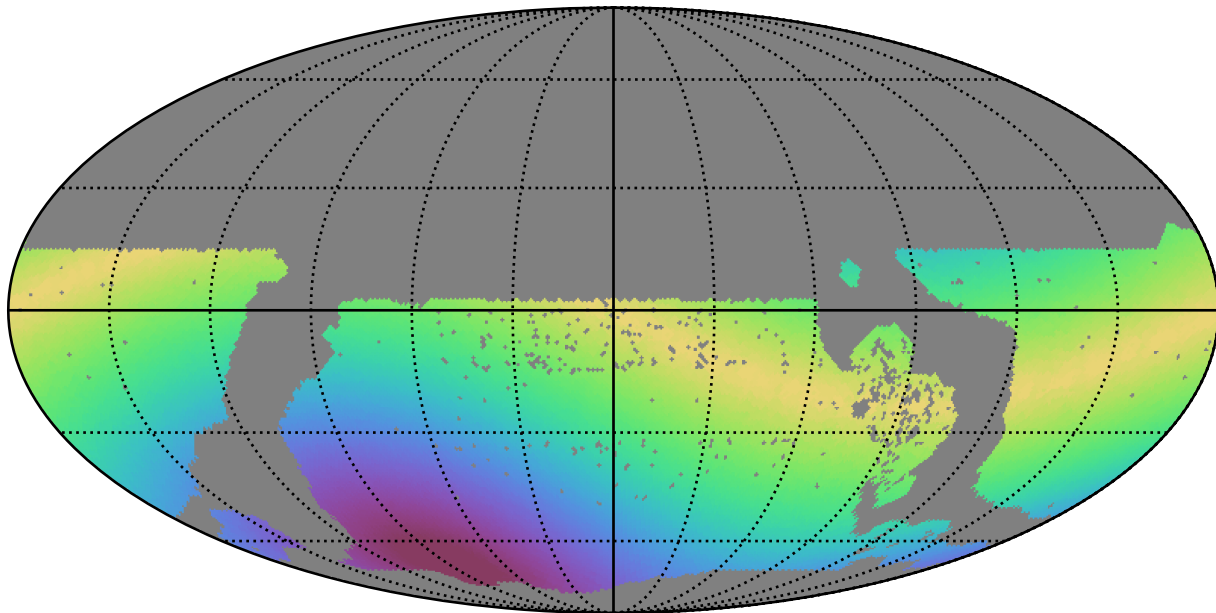
too_elab_r64_d2_gz_v3.4_10yrs WFD y band: Max solarElong
