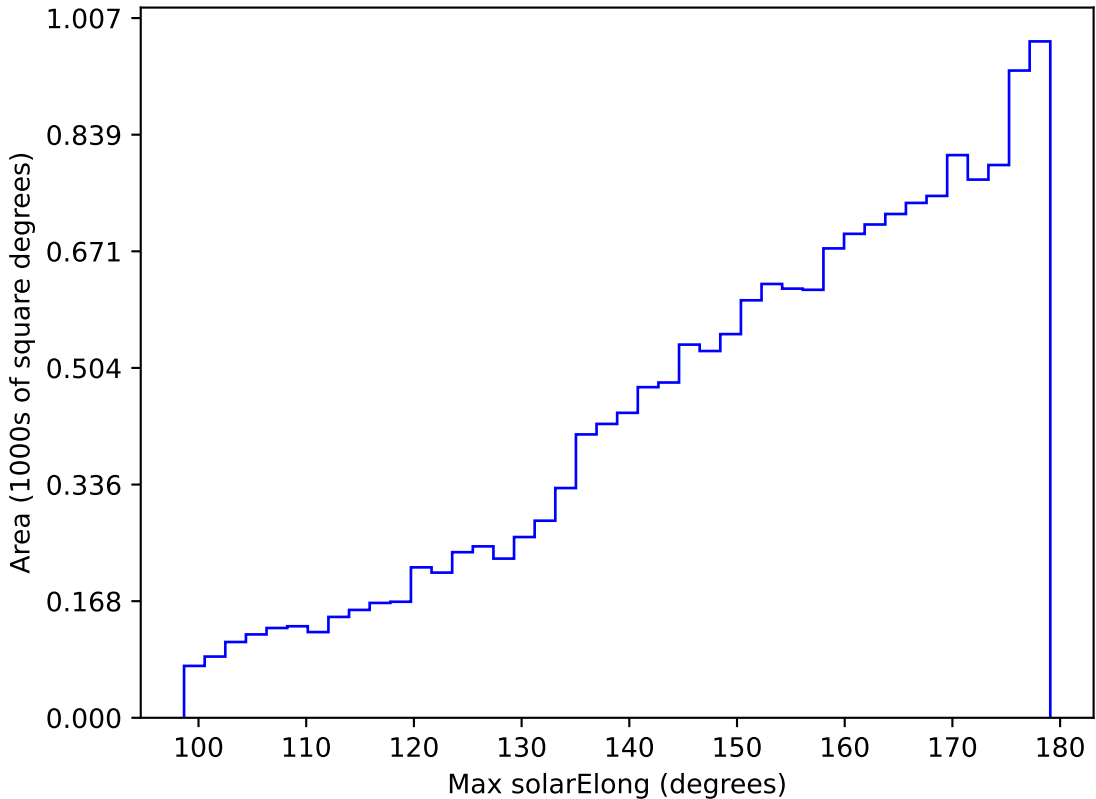
too_elab_r64_d2_gz_v3.4_10yrs WFD y band: Max solarElong
