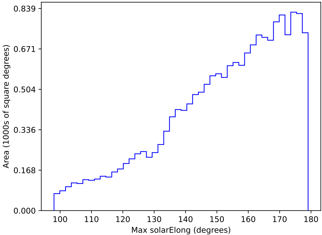
too_elab_r64_d2_gz_v3.4_10yrs WFD u band: Max solarElong
