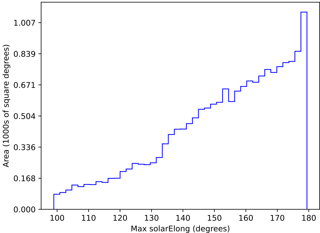
too_elab_r64_d2_gz_v3.4_10yrs WFD i band: Max solarElong
