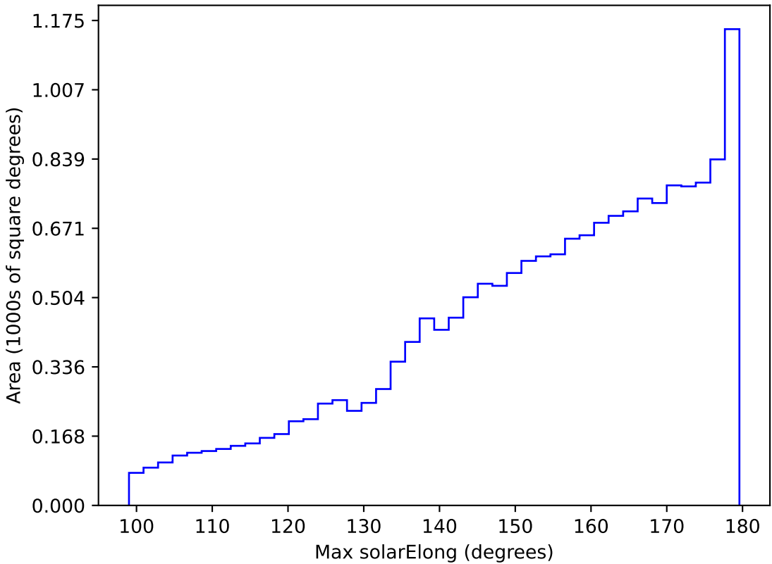
too_elab_r64_d2_gz_v3.4_10yrs WFD all bands: Max solarElong
