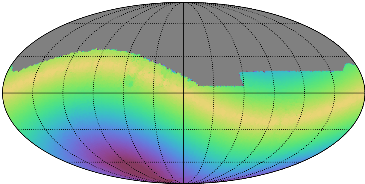
too_elab_r64_d2_gz_v3.4_10yrs All sky z band: Max solarElong
