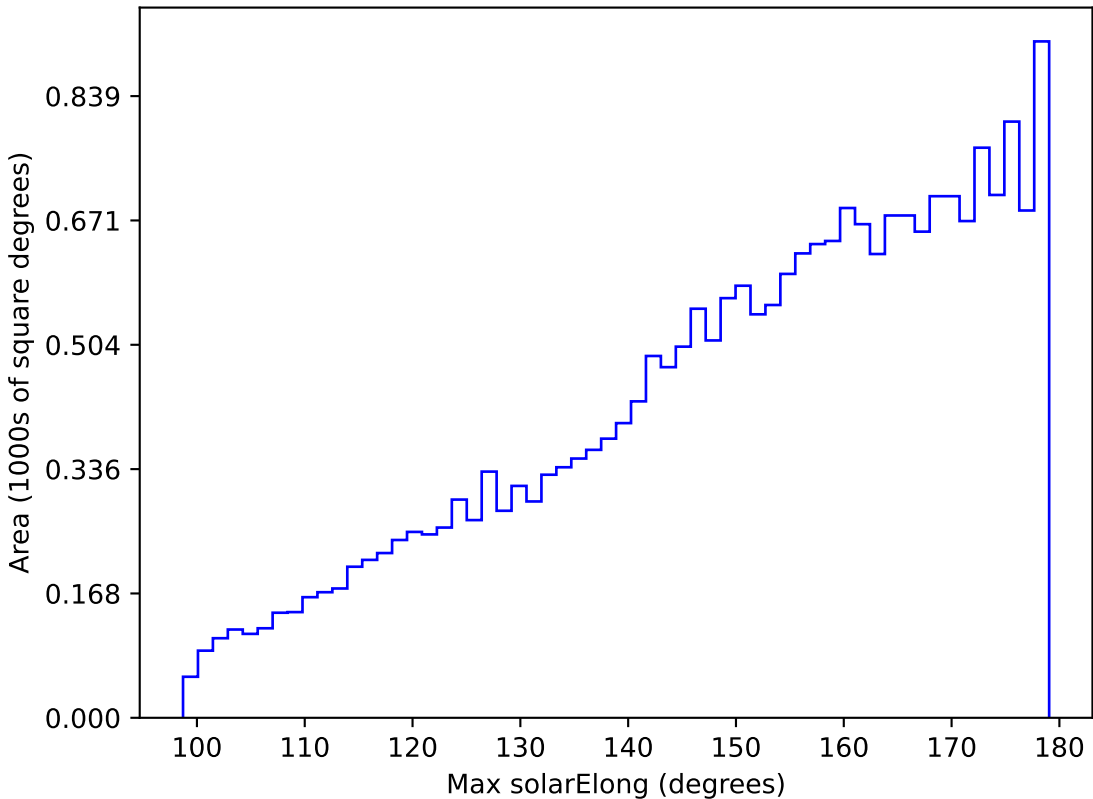
too_elab_r64_d2_gz_v3.4_10yrs All sky y band: Max solarElong
