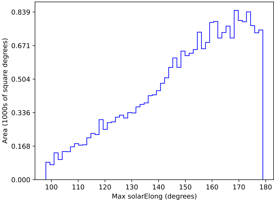
too_elab_r64_d2_gz_v3.4_10yrs All sky u band: Max solarElong
