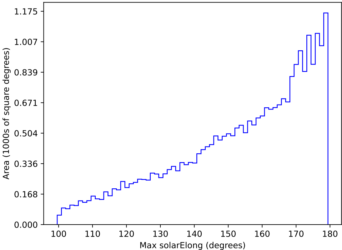
too_elab_r64_d2_gz_v3.4_10yrs All sky r band: Max solarElong
