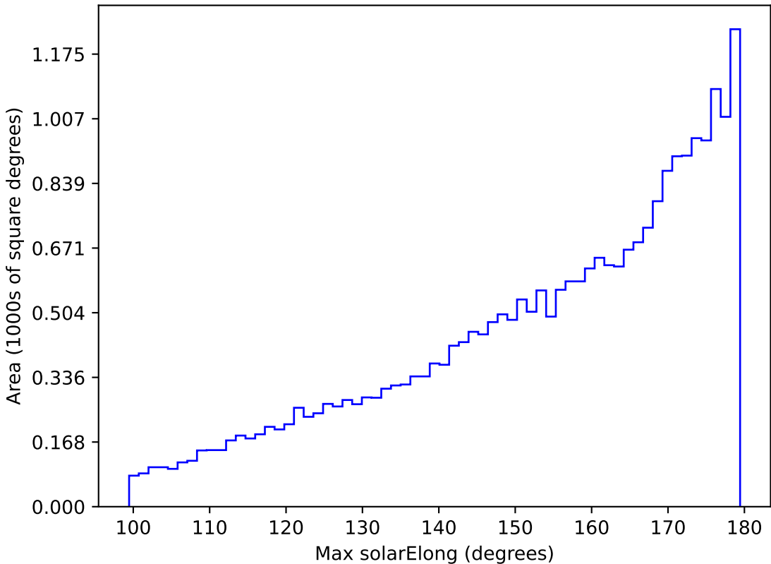
too_elab_r64_d2_gz_v3.4_10yrs All sky i band: Max solarElong
