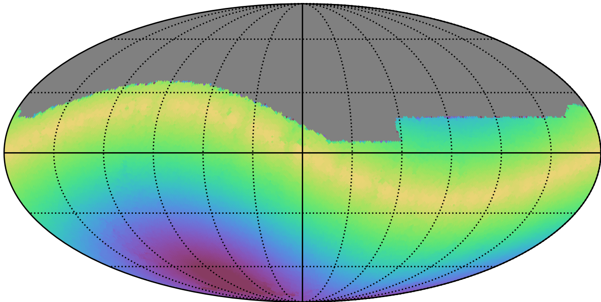
too_elab_r64_d2_gz_v3.4_10yrs All sky g band: Max solarElong
