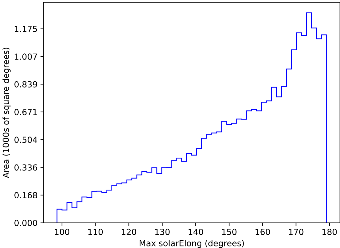
too_elab_r64_d2_gz_v3.4_10yrs All sky g band: Max solarElong
