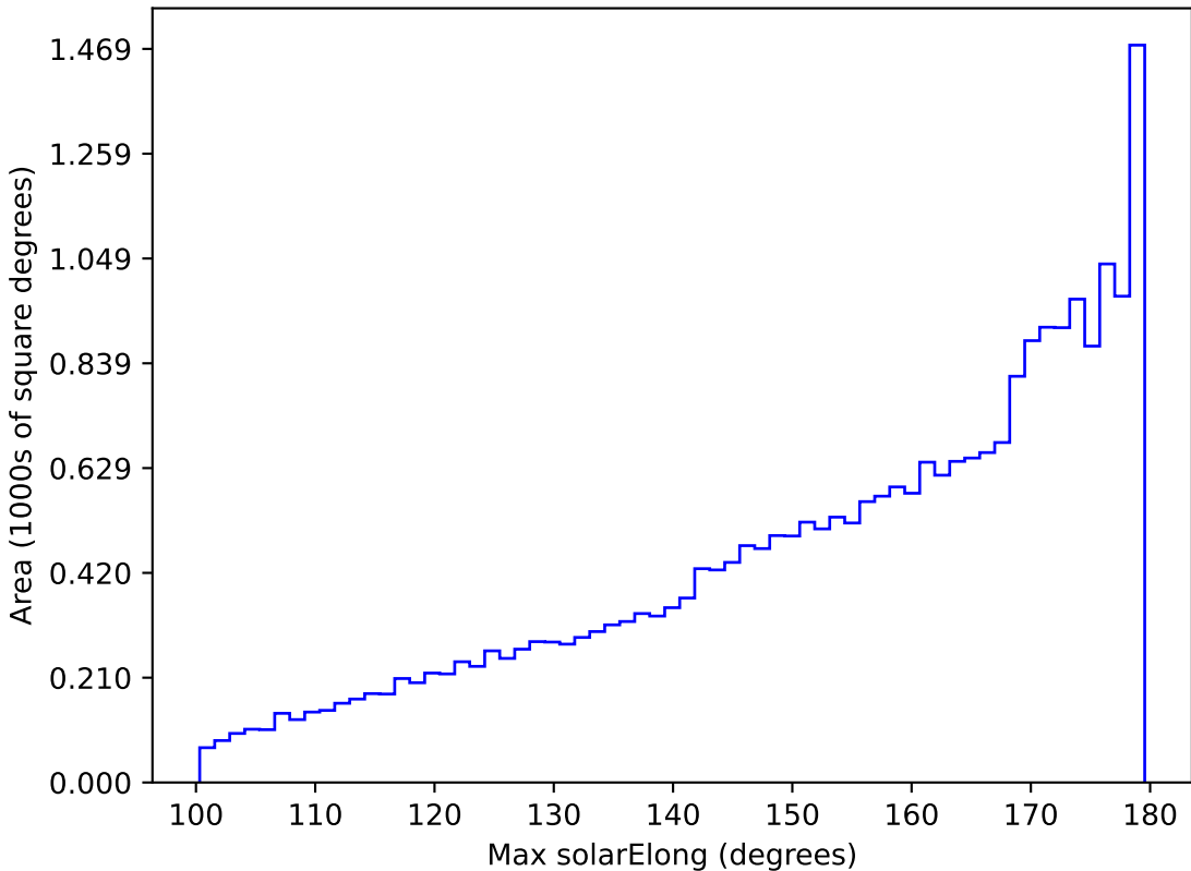
too_elab_r64_d2_gz_v3.4_10yrs All sky all bands: Max solarElong
