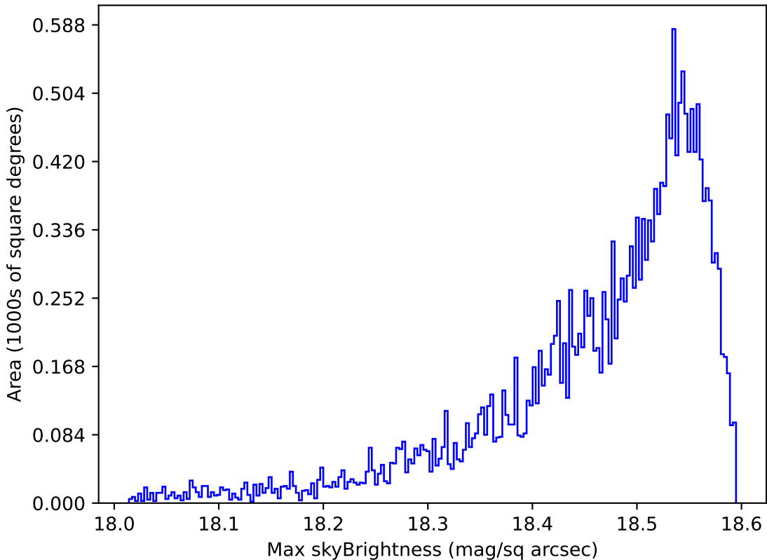
too_elab_r64_d2_gz_v3.4_10yrs Yr 1 y band: Max skyBrightness
