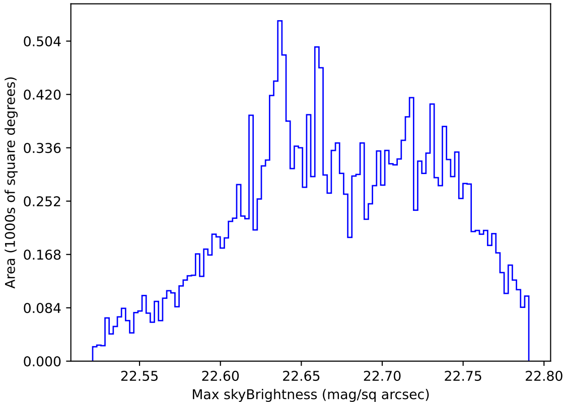
too_elab_r64_d2_gz_v3.4_10yrs Yr 1 u band: Max skyBrightness
