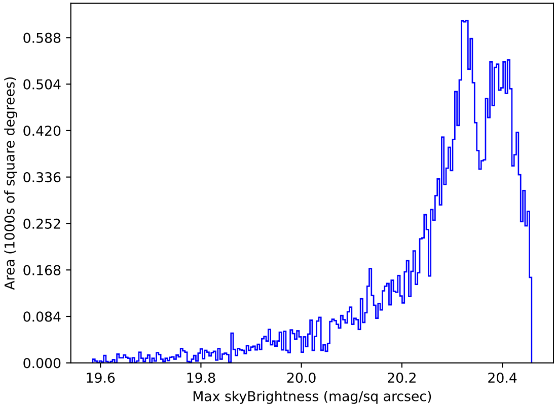
too_elab_r64_d2_gz_v3.4_10yrs Yr 1 i band: Max skyBrightness
