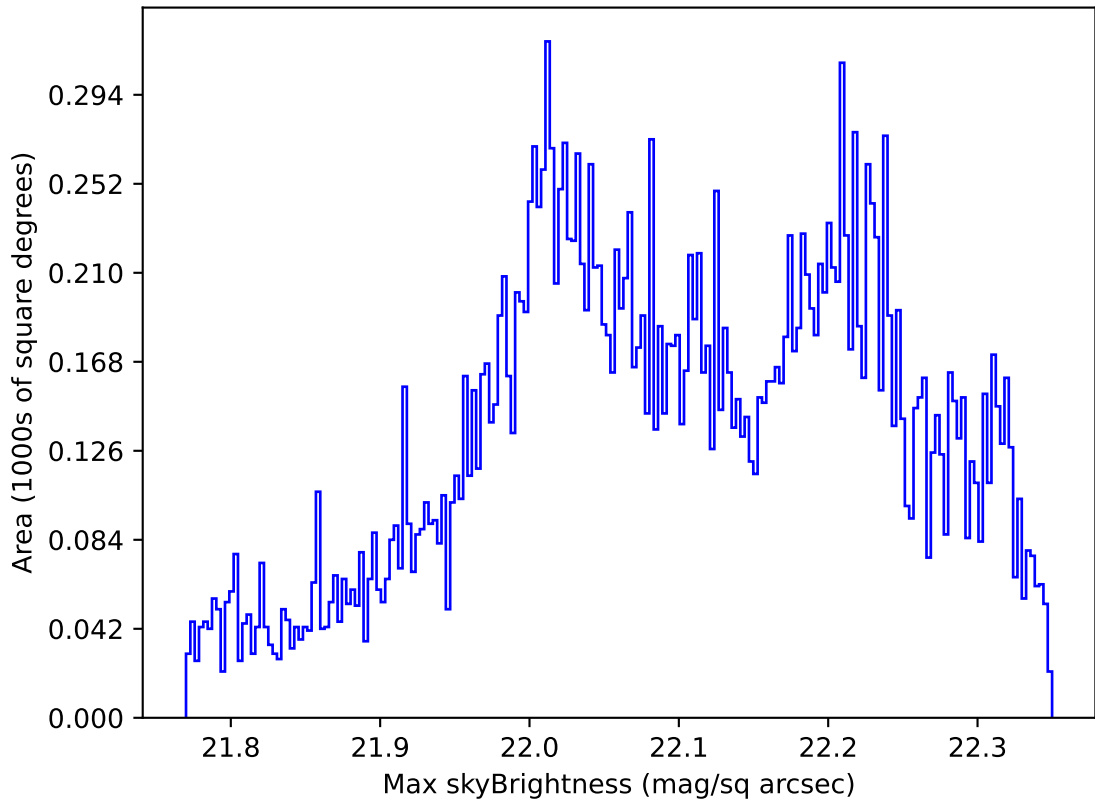
too_elab_r64_d2_gz_v3.4_10yrs Yr 1 g band: Max skyBrightness
