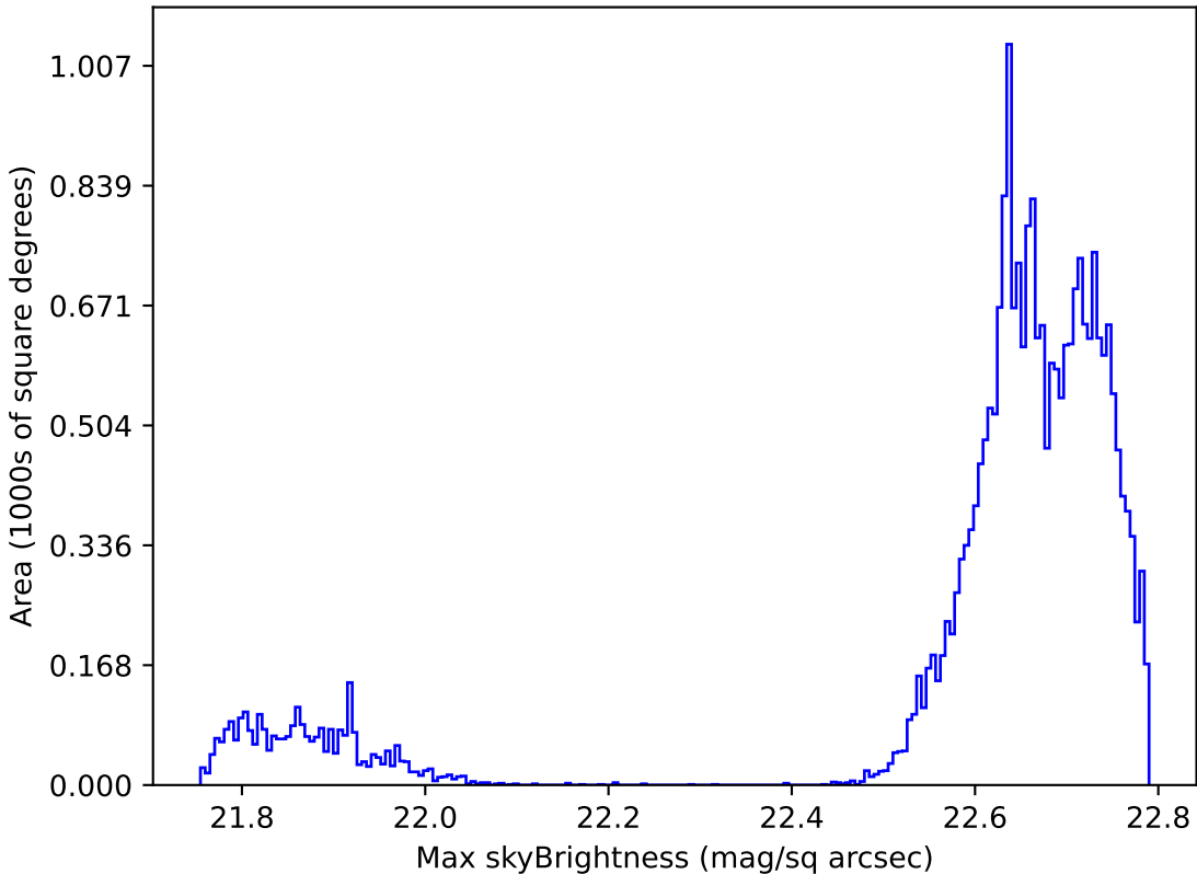
too_elab_r64_d2_gz_v3.4_10yrs Yr 1 all bands: Max skyBrightness
