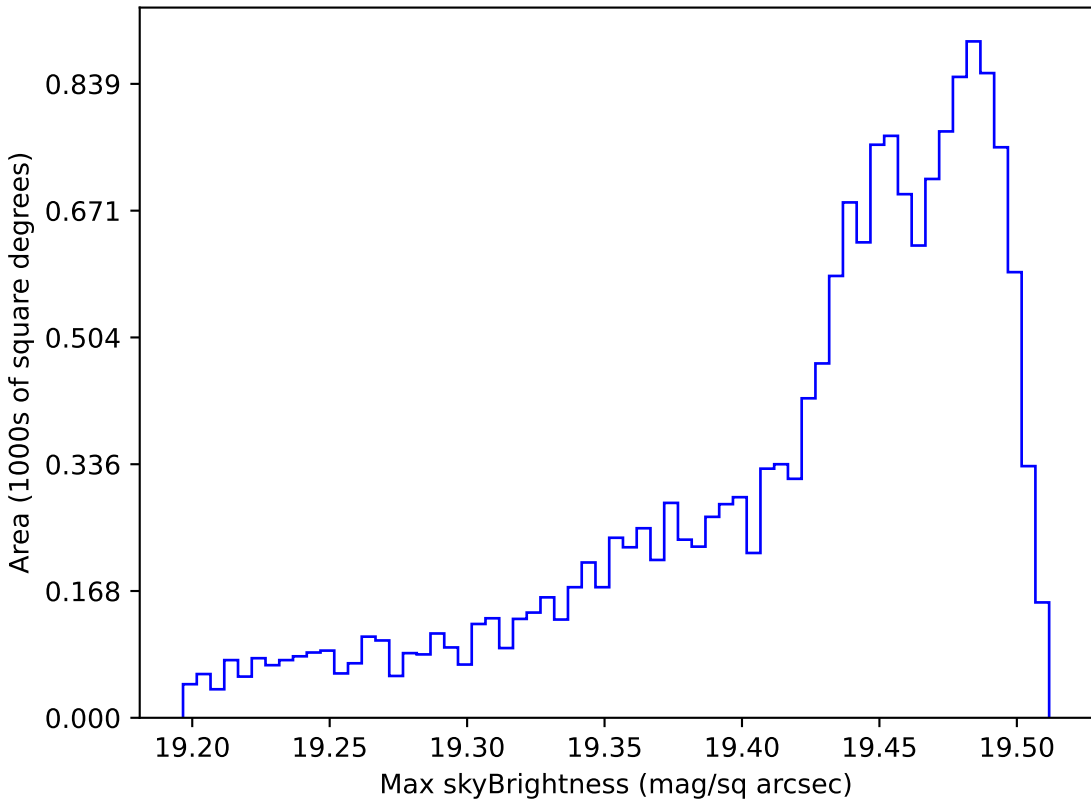
too_elab_r64_d2_gz_v3.4_10yrs WFD z band: Max skyBrightness
