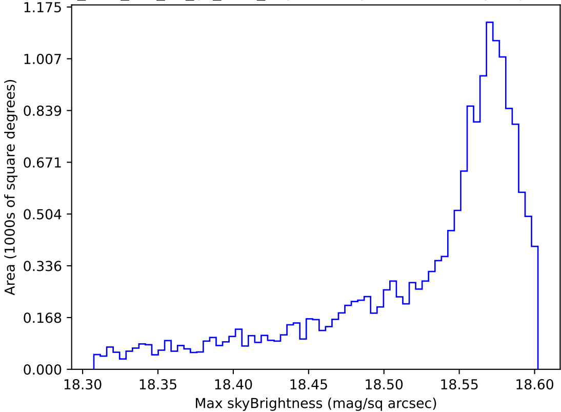
too_elab_r64_d2_gz_v3.4_10yrs WFD y band: Max skyBrightness
