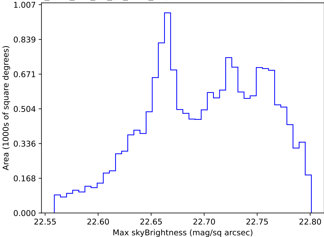
too_elab_r64_d2_gz_v3.4_10yrs WFD u band: Max skyBrightness
