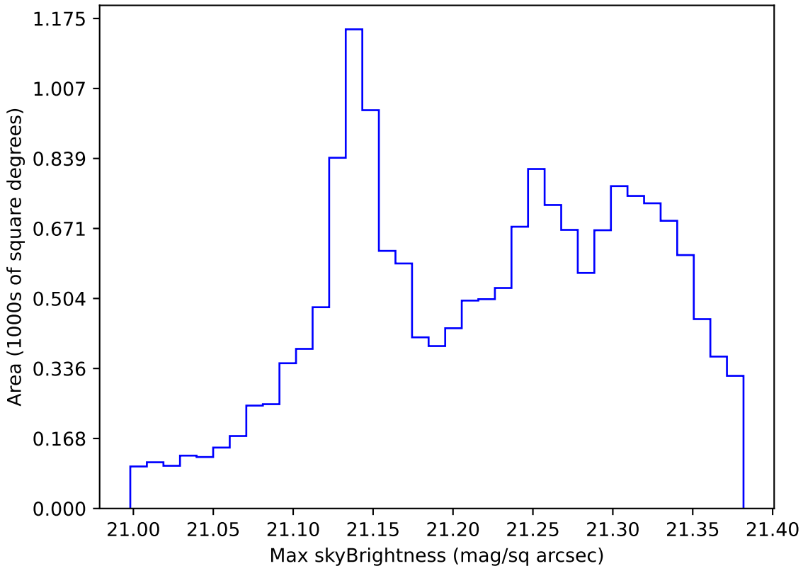
too_elab_r64_d2_gz_v3.4_10yrs WFD r band: Max skyBrightness
