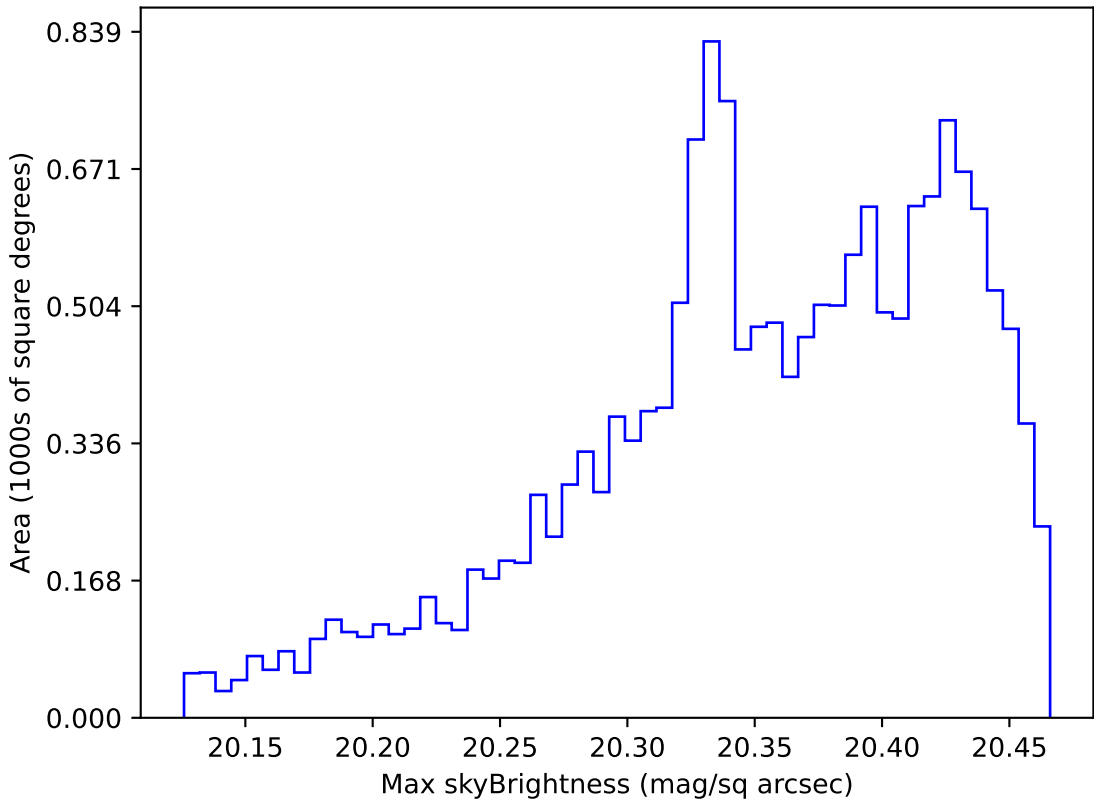
too_elab_r64_d2_gz_v3.4_10yrs WFD i band: Max skyBrightness
