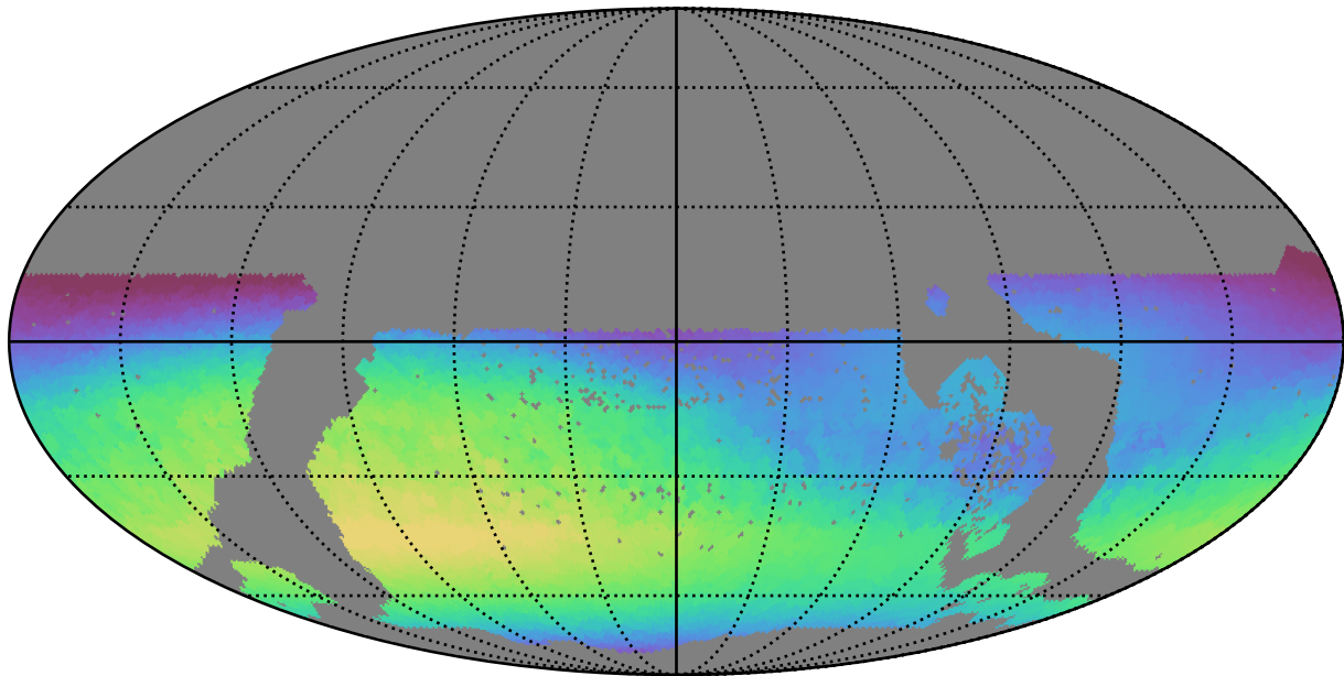
too_elab_r64_d2_gz_v3.4_10yrs WFD all bands: Max skyBrightness
