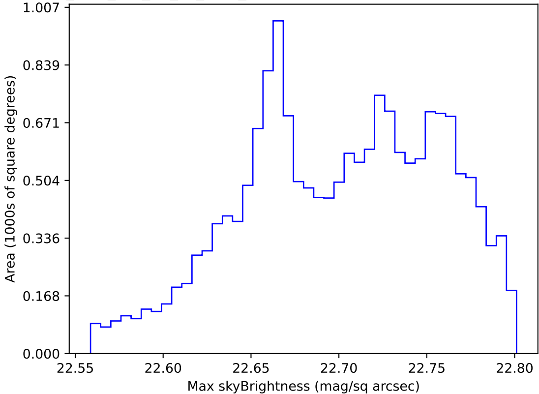
too_elab_r64_d2_gz_v3.4_10yrs WFD all bands: Max skyBrightness
