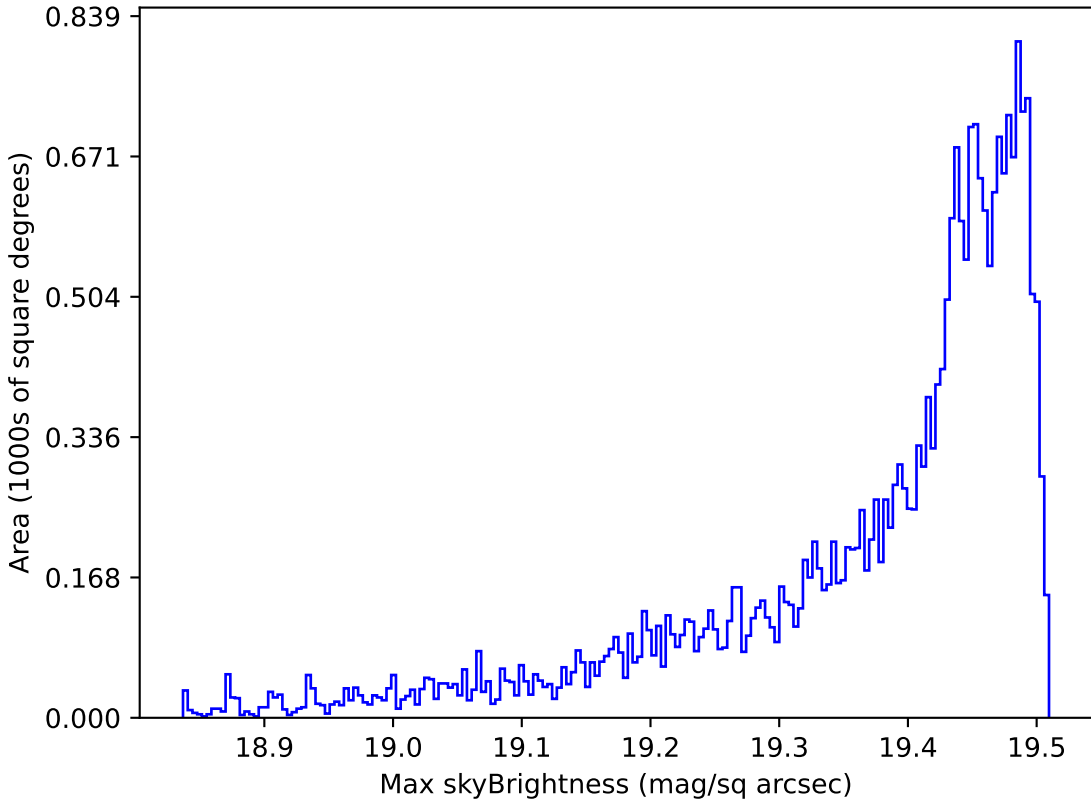
too_elab_r64_d2_gz_v3.4_10yrs All sky z band: Max skyBrightness
