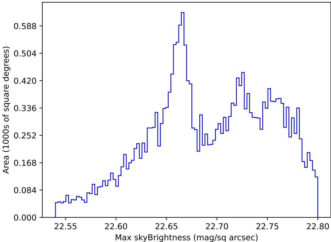
too_elab_r64_d2_gz_v3.4_10yrs All sky u band: Max skyBrightness
