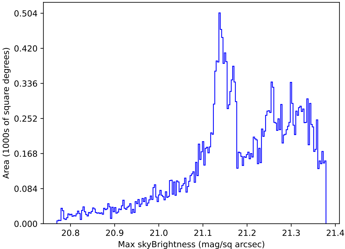
too_elab_r64_d2_gz_v3.4_10yrs All sky r band: Max skyBrightness
