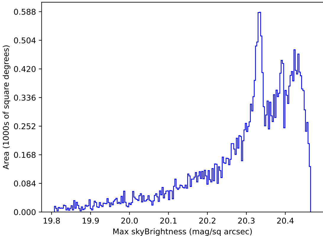
too_elab_r64_d2_gz_v3.4_10yrs All sky i band: Max skyBrightness
