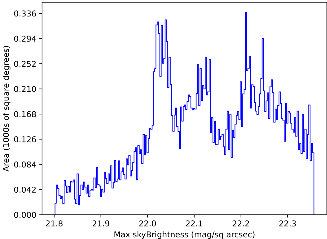
too_elab_r64_d2_gz_v3.4_10yrs All sky g band: Max skyBrightness
