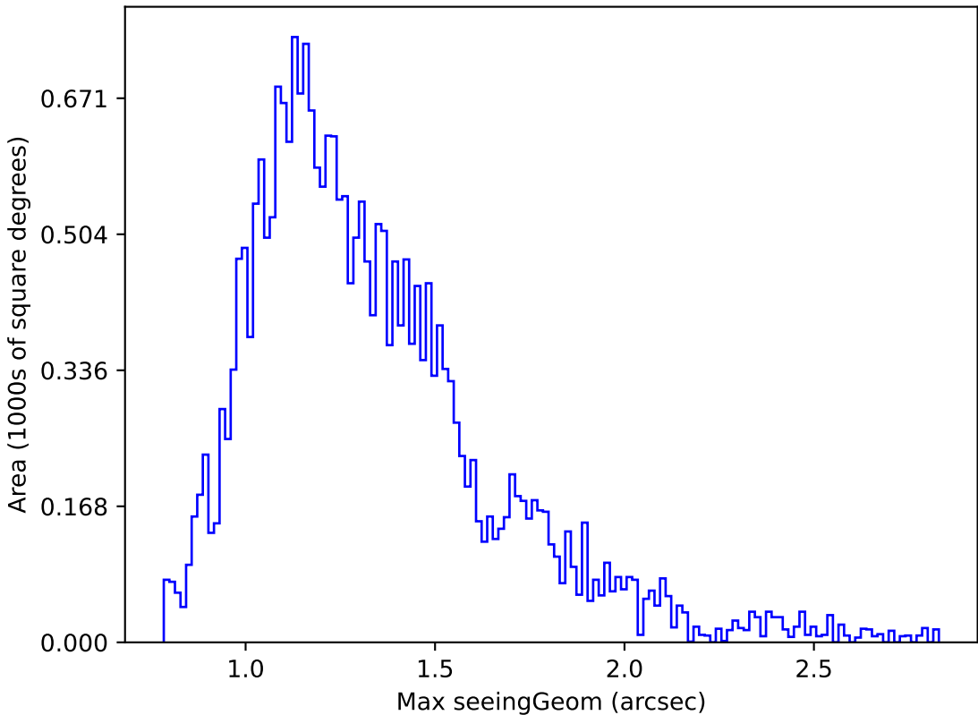
too_elab_r64_d2_gz_v3.4_10yrs Yr 1 z band: Max seeingGeom
