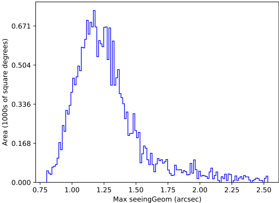
too_elab_r64_d2_gz_v3.4_10yrs Yr 1 y band: Max seeingGeom
