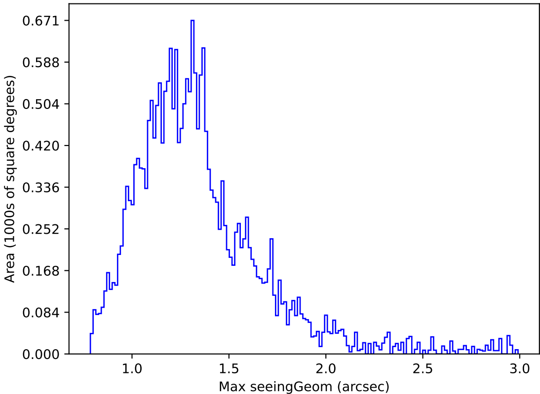
too_elab_r64_d2_gz_v3.4_10yrs Yr 1 u band: Max seeingGeom
