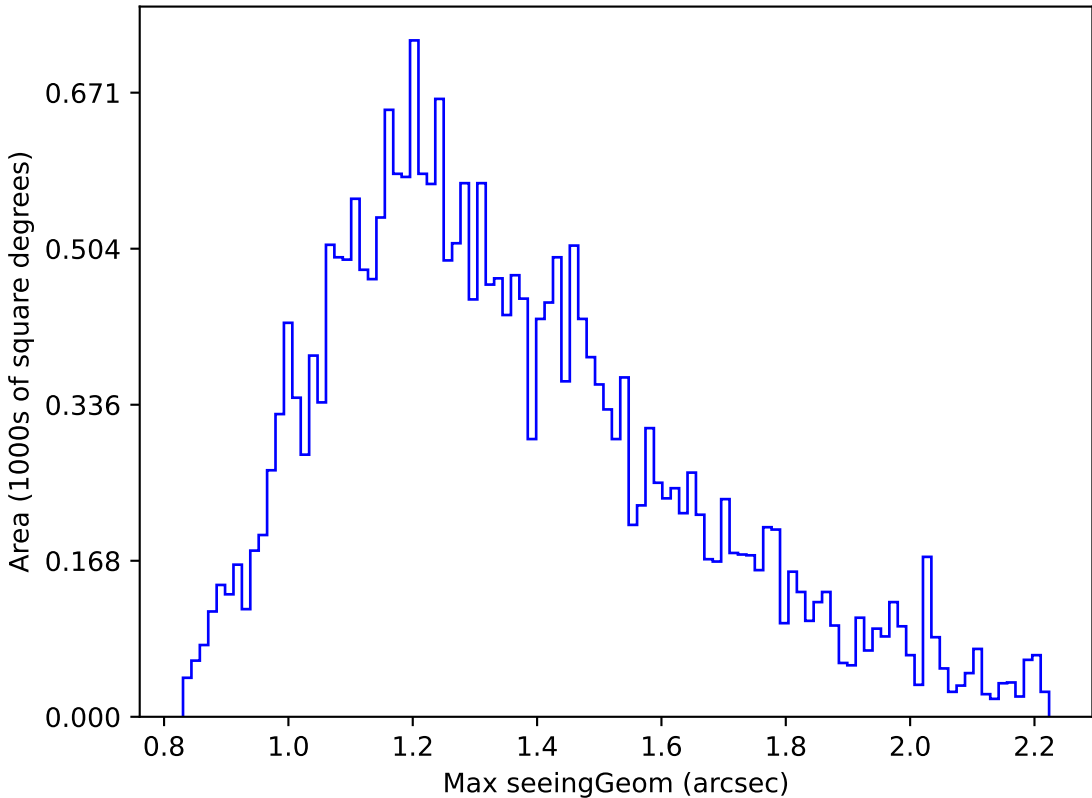
too_elab_r64_d2_gz_v3.4_10yrs Yr 1 r band: Max seeingGeom
