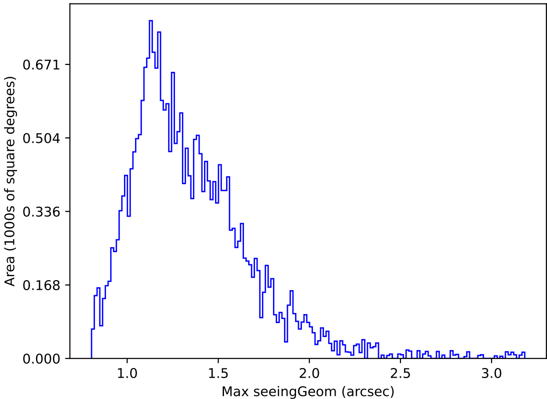
too_elab_r64_d2_gz_v3.4_10yrs Yr 1 g band: Max seeingGeom
